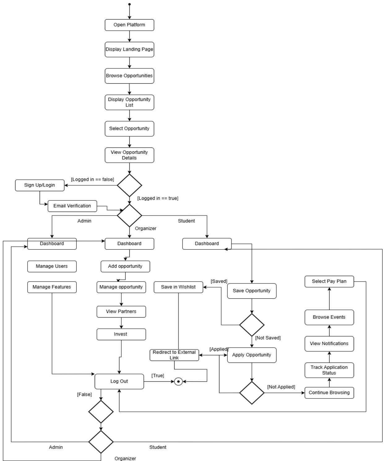
Fig. 4: Activity Diagram
