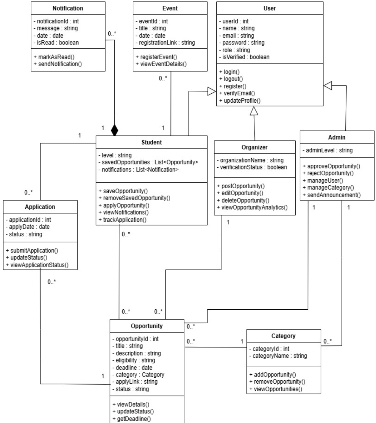
Fig 3: Class Diagram
